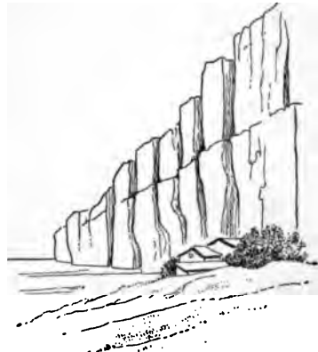
FIG. 216.—Cliffs in loess 200 feet in height which exhibit the characteristic vertical jointing (after von Richtofen).
